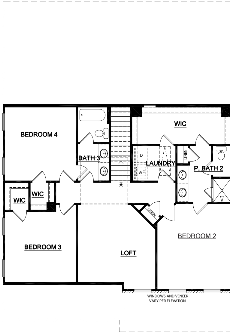
SECOND FLOOR
